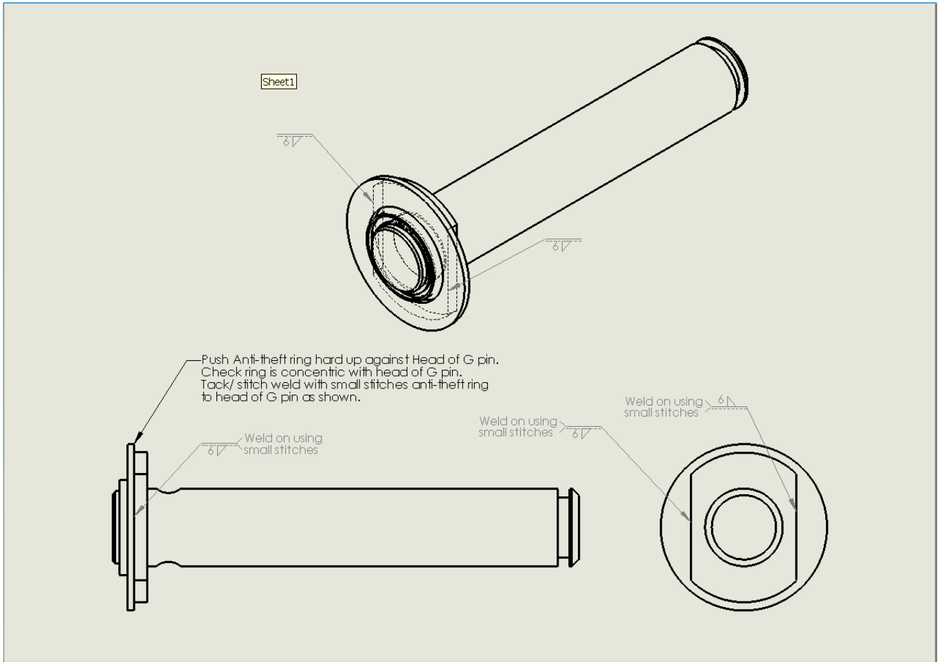
Figure 2: Positioning of anti-theft ring onto G pin.
