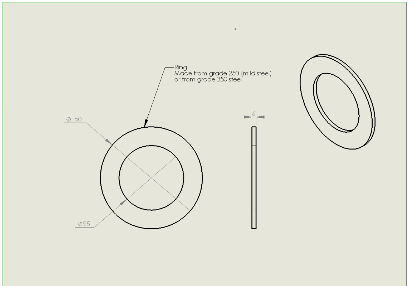
Figure 1: Ring to be cut from steel plate.
